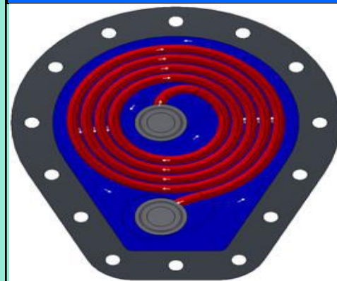
Figure 1. Spiral Flow Path
